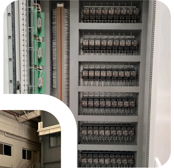
Relay Panel
